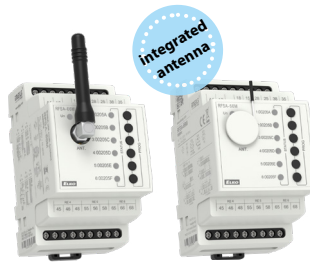
RFSA-66M RFSA-66MI Switch units, 6 channels – multifunction, 6x 8 A
