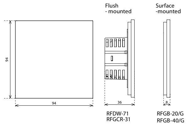
Flush - mounted
